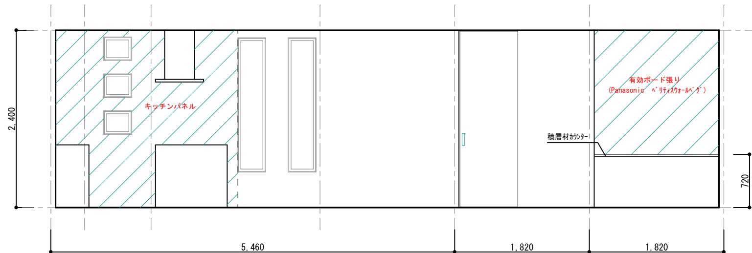
LDK
